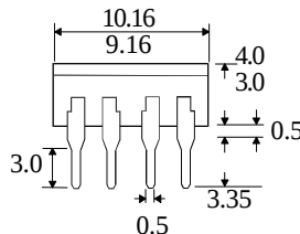
TLP521-4
